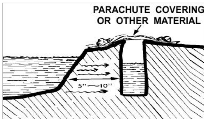
Figure IX-5. Filtration Systems, Settling Water
